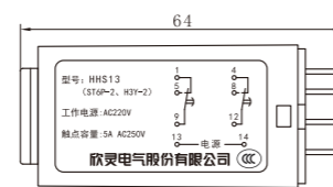
HHS13 (ST6P-2、H3Y-2)
