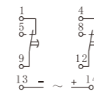
HHS13 (ST6P-2、H3Y-2)
