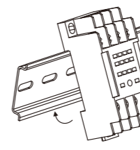
(7) 将底座扣入导轨
