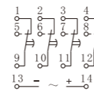
HHS13-1 (ST6P-4、H3Y-4)
